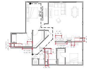
UNIT TYPE 2-2B: FLOOR PLAN
