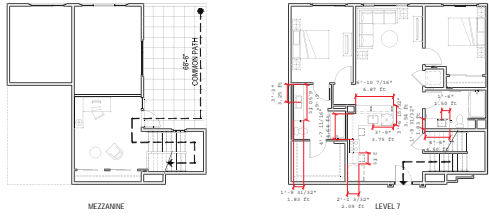
UNIT TYPE 2-1CL: FLOOR PLAN
