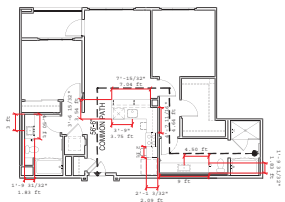
UNIT TYPE 2-1B: FLOOR PLAN
