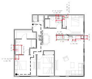
UNIT TYPE 3-1: FLOOR PLAN
