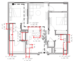
UNIT TYPE 2-1: FLOOR PLAN
