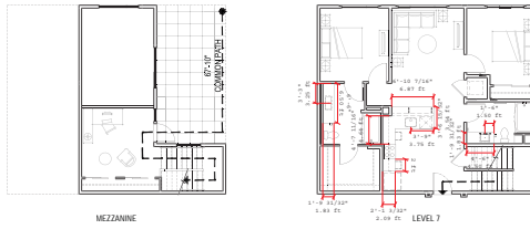
UNIT TYPE 2-1LX: FLOOR PLAN
