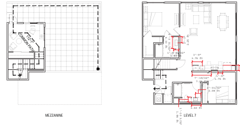
UNIT TYPE 2-2ALL: FLOOR PLAN
