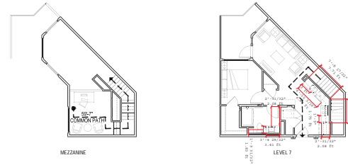
UNIT TYPE 1-2L: FLOOR PLAN
