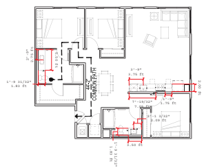
UNIT TYPE 3-2: FLOOR PLAN
