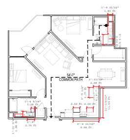
UNIT TYPE 2-3: FLOOR PLAN
