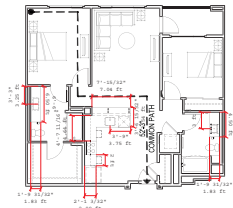
UNIT TYPE 2-1C: FLOOR PLAN
