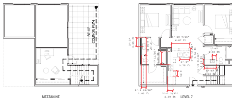
UNIT TYPE 2-1L: FLOOR PLAN
