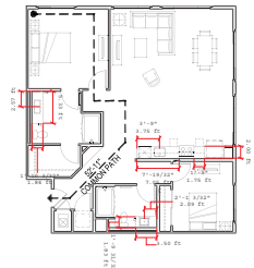
UNIT TYPE 2-2A: FLOOR PLAN
