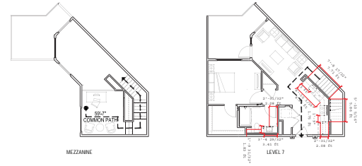
UNIT TYPE 2-2AL: FLOOR PLAN
