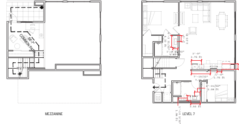
UNIT TYPE 2-2AL: FLOOR PLAN
