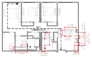
UNIT TYPE 3-3: FLOOR PLAN
