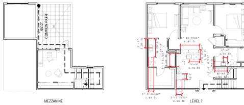
UNIT TYPE 2-1LL: FLOOR PLAN
